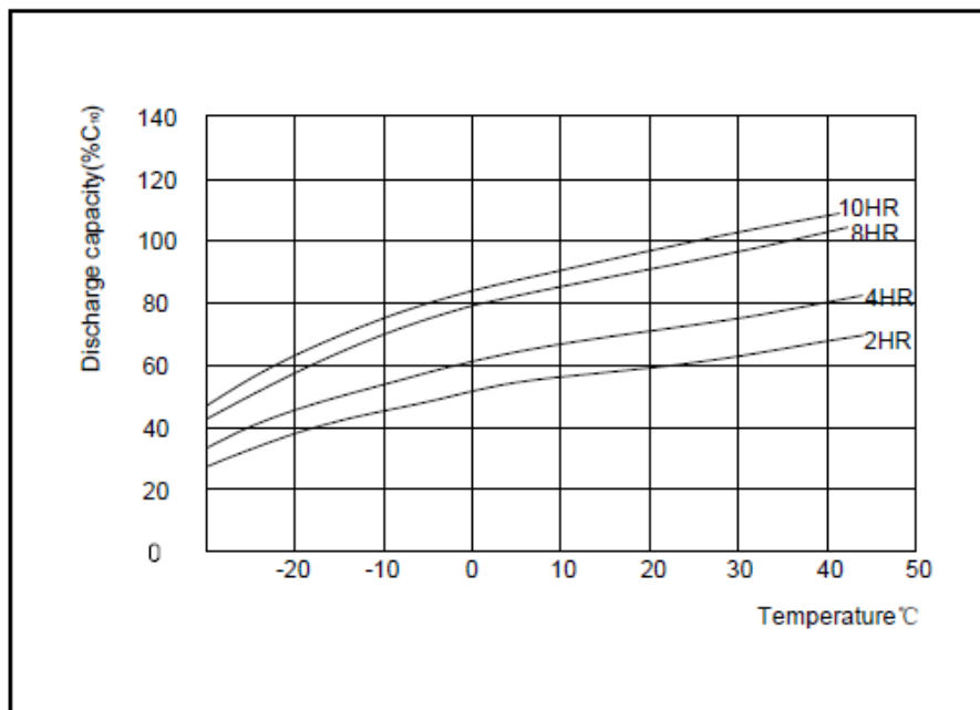
Capacity at Different Temperature
