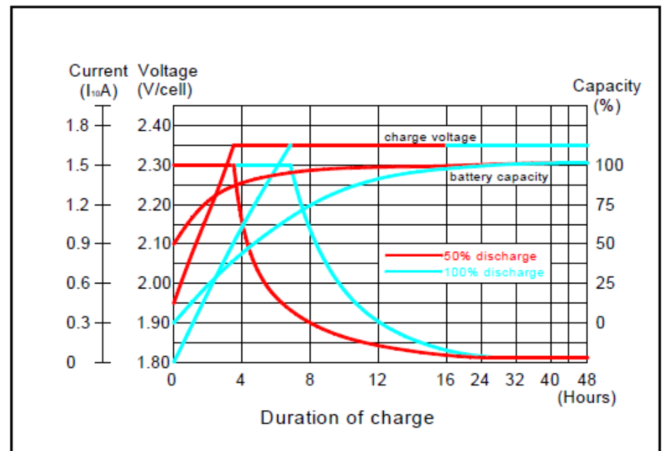
Constant Voltage Charge Characteristics
